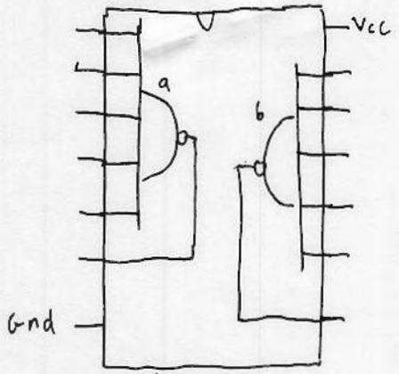
MC1800 Dual 5-input NAND Gate (DTL)
