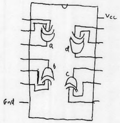
74L86 (Not as 7486) Quad XOR gate
