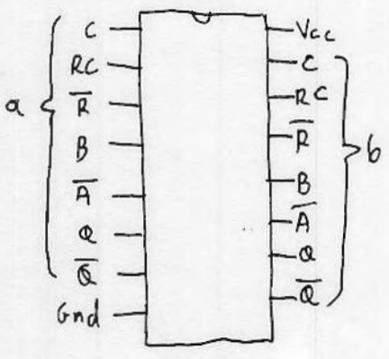
9602 Dual Retriggerable Monostable
