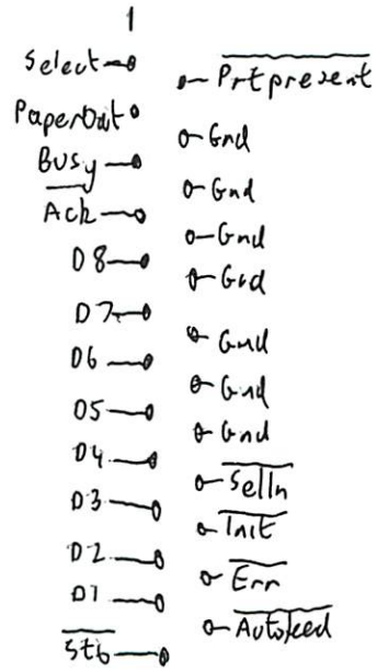
Parallel Port DB25 plug
