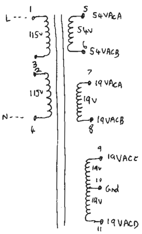
Mains Transformer
