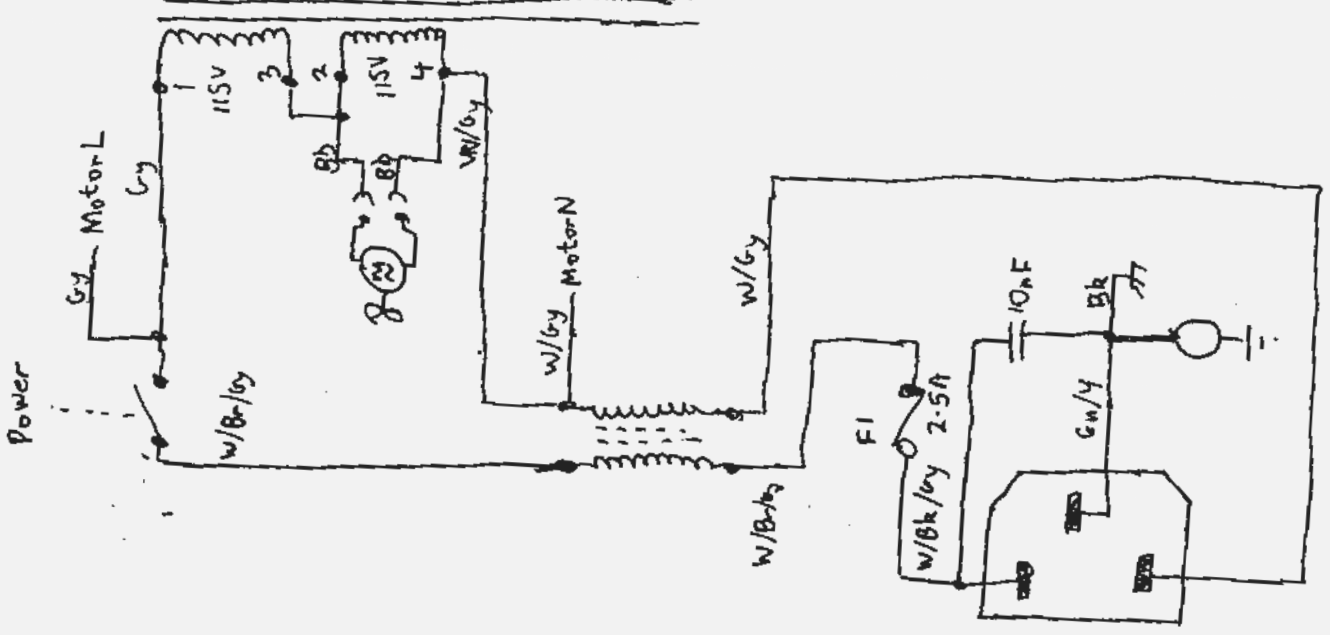
MD7768A Chassis Wiring Sheet ①
